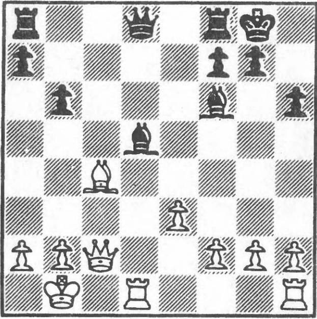
459 After 16 Bc4
